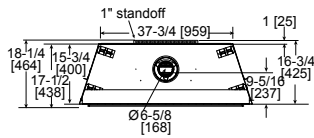
RAVE4013I Dimensions
